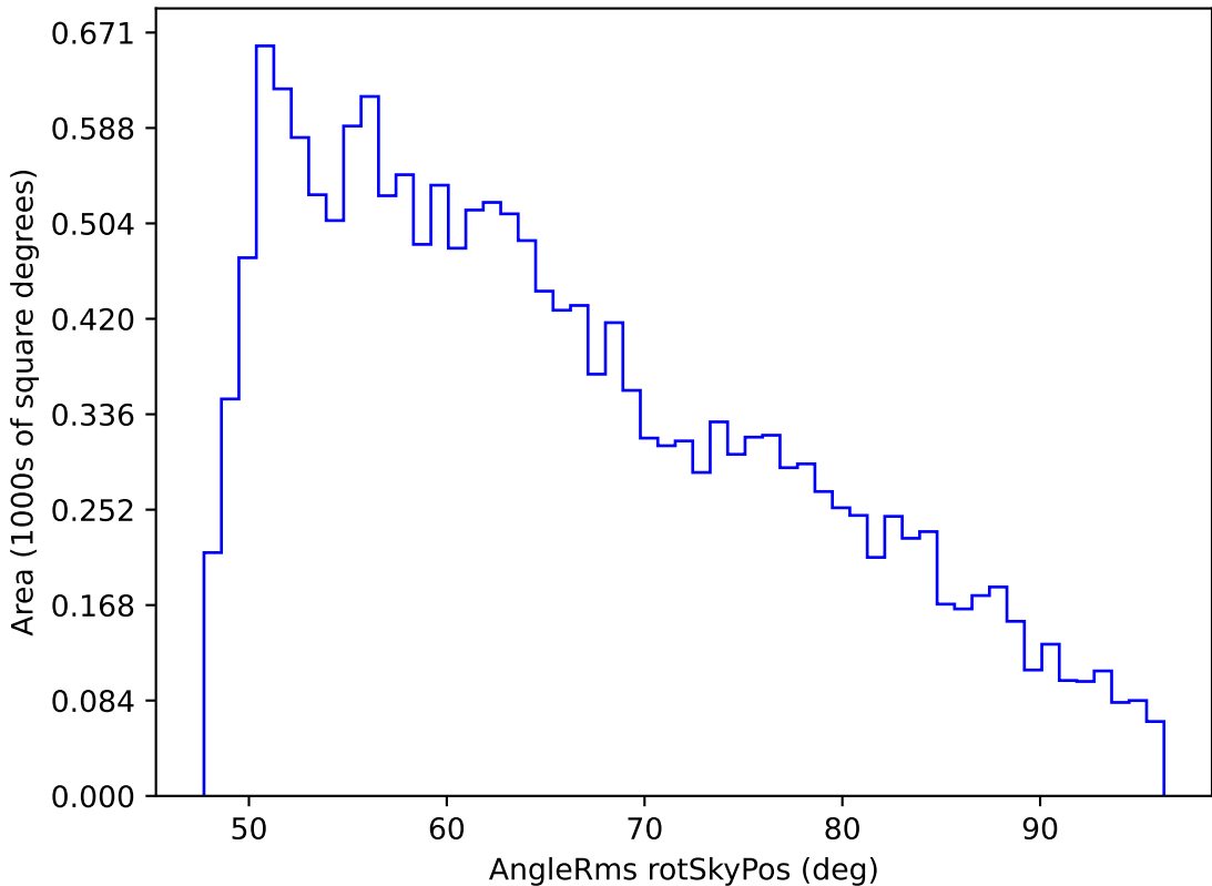
noroll_mjdp270_v3.4_10yrs WFD i band: AngleRms rotSkyPos
