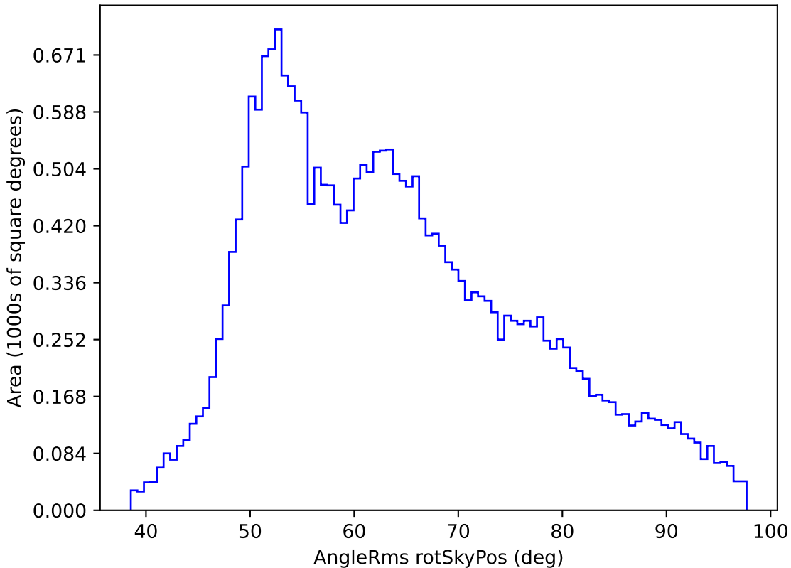
noroll_mjdp270_v3.4_10yrs All sky z band: AngleRms rotSkyPos
