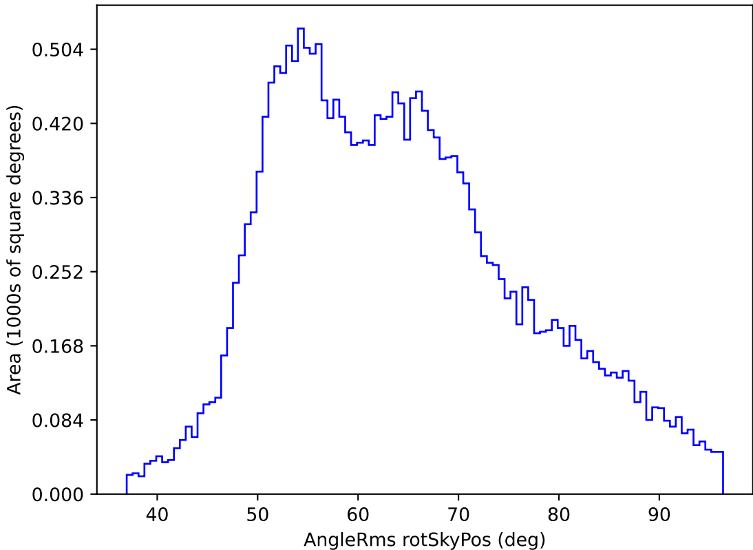
noroll_mjdp270_v3.4_10yrs All sky y band: AngleRms rotSkyPos
