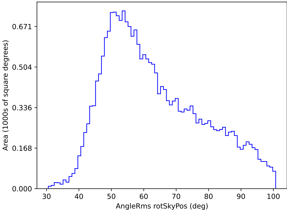
noroll_mjdp270_v3.4_10yrs All sky u band: AngleRms rotSkyPos
