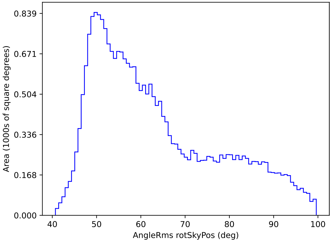
noroll_mjdp270_v3.4_10yrs All sky r band: AngleRms rotSkyPos
