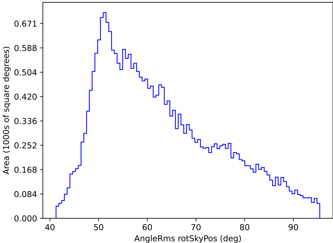
noroll_mjdp270_v3.4_10yrs All sky i band: AngleRms rotSkyPos
