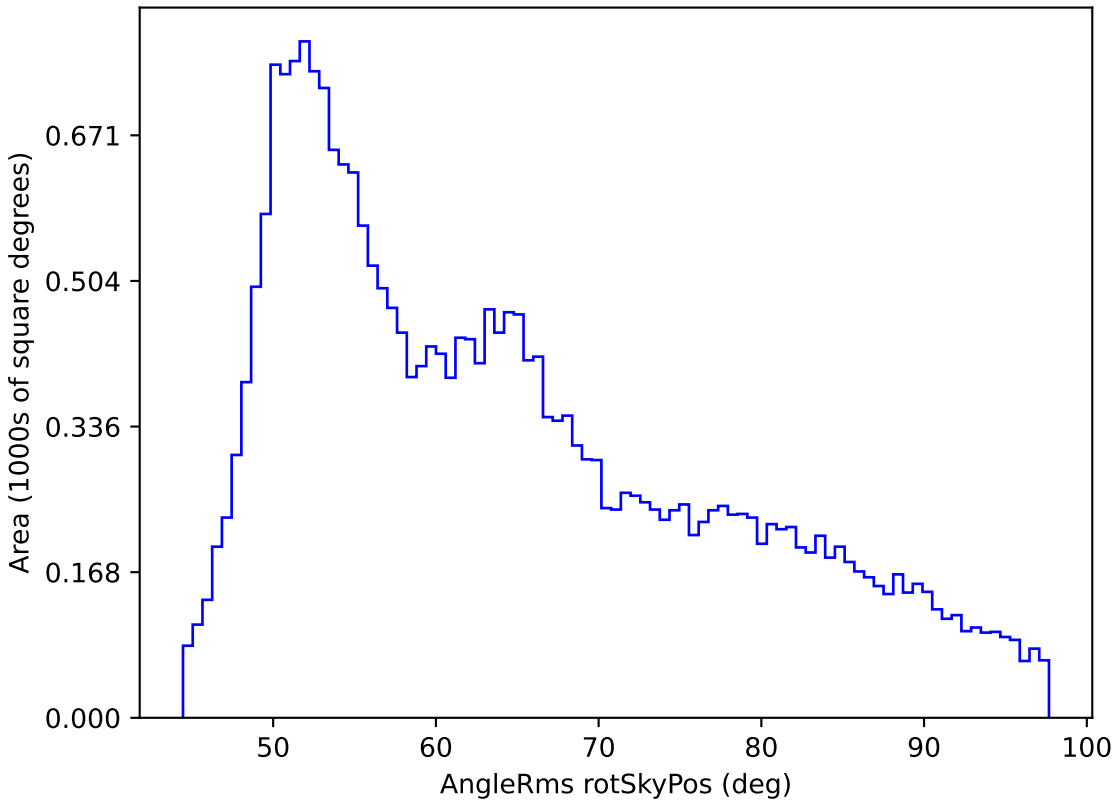
noroll_mjdp270_v3.4_10yrs All sky all bands: AngleRms rotSkyPos
