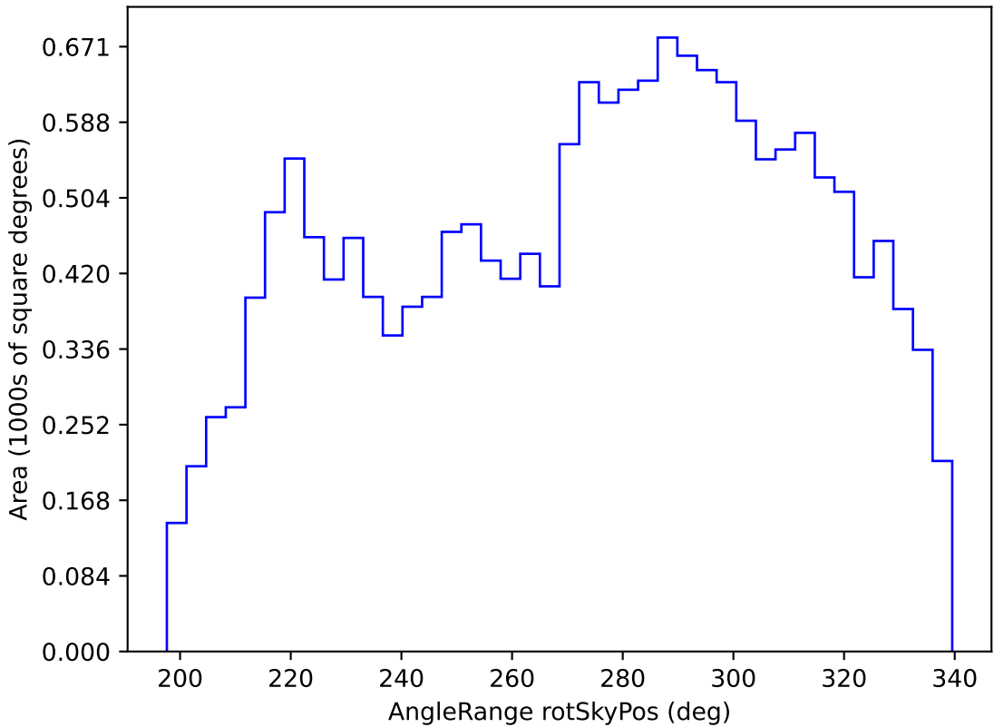
noroll_mjdp270_v3.4_10yrs WFD y band: AngleRange rotSkyPos
