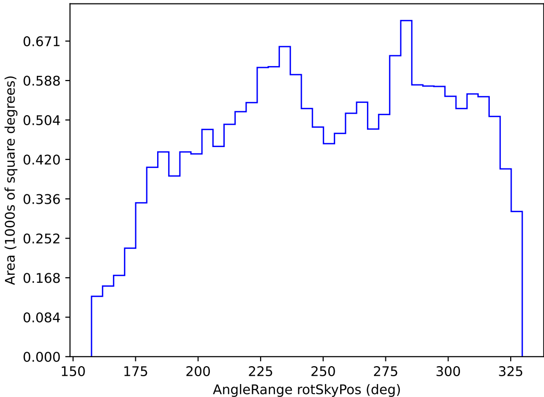
noroll_mjdp270_v3.4_10yrs WFD u band: AngleRange rotSkyPos
