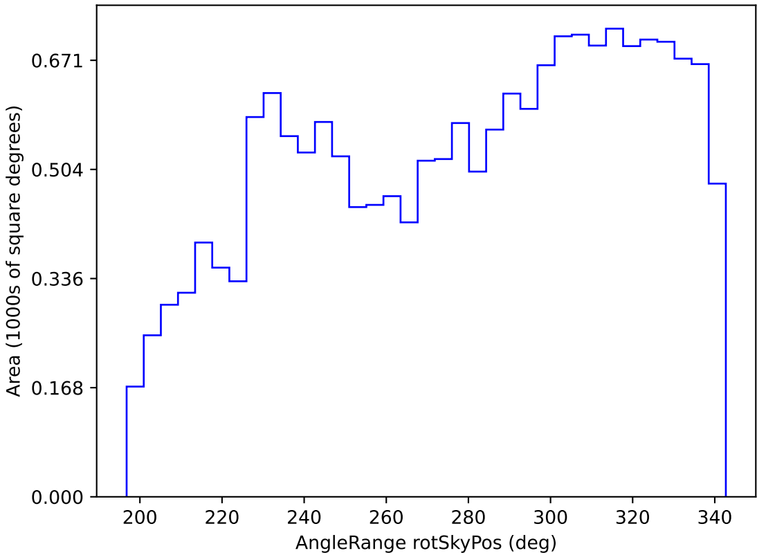
noroll_mjdp270_v3.4_10yrs WFD i band: AngleRange rotSkyPos
