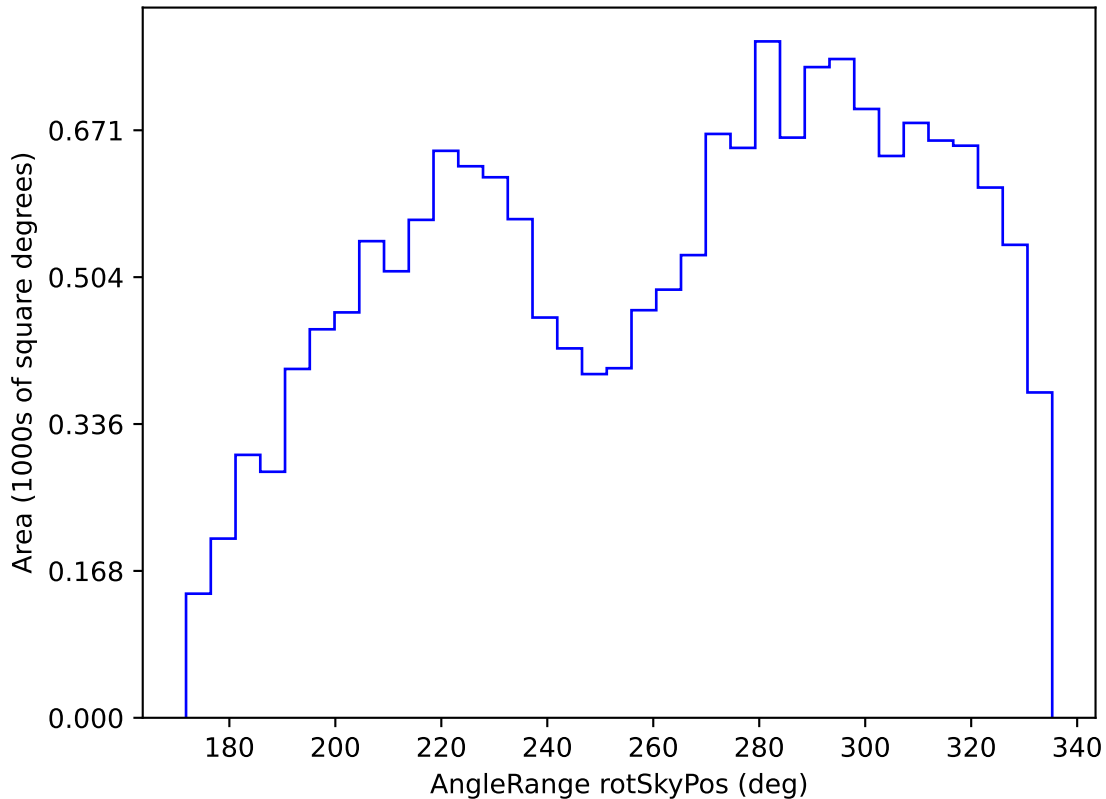
noroll_mjdp270_v3.4_10yrs WFD g band: AngleRange rotSkyPos
