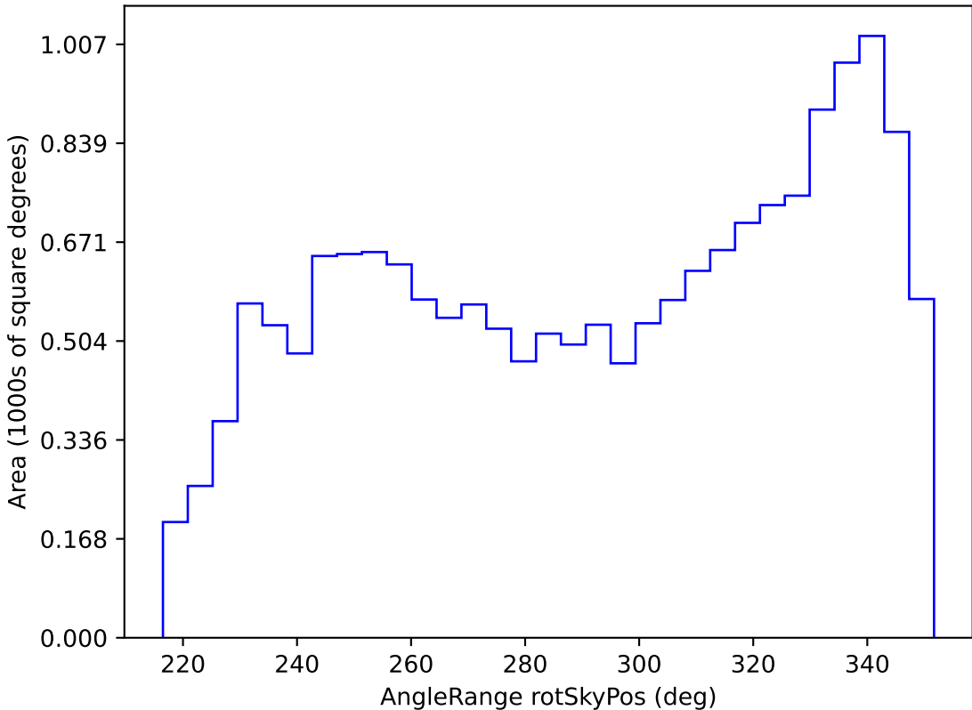
noroll_mjdp270_v3.4_10yrs WFD all bands: AngleRange rotSkyPos
