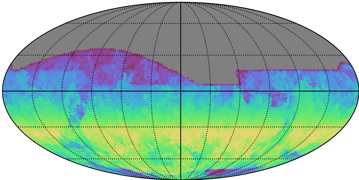
noroll_mjdp270_v3.4_10yrs All sky z band: AngleRange rotSkyPos
