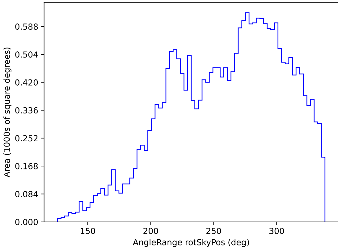
noroll_mjdp270_v3.4_10yrs All sky y band: AngleRange rotSkyPos
