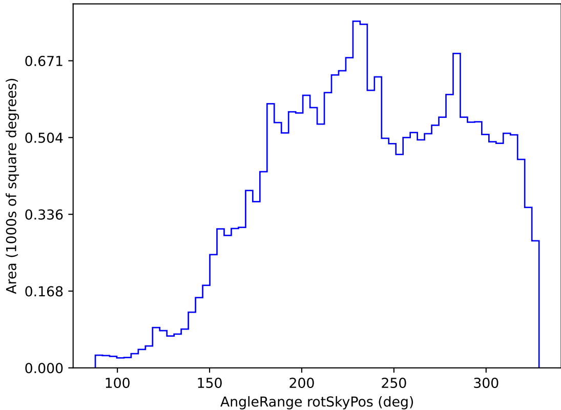
noroll_mjdp270_v3.4_10yrs All sky u band: AngleRange rotSkyPos
