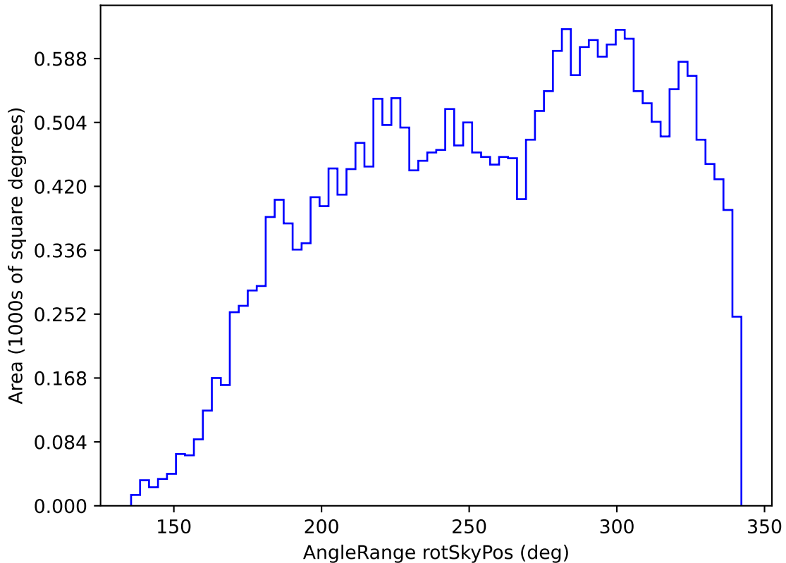
noroll_mjdp270_v3.4_10yrs All sky r band: AngleRange rotSkyPos
