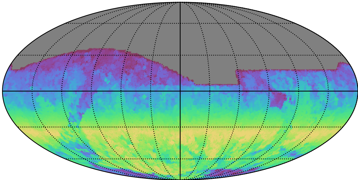
noroll_mjdp270_v3.4_10yrs All sky i band: AngleRange rotSkyPos
