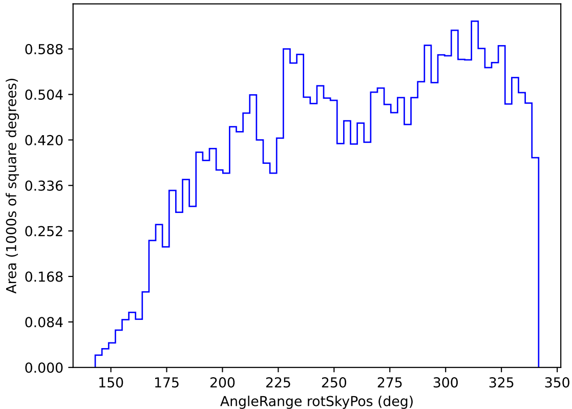
noroll_mjdp270_v3.4_10yrs All sky i band: AngleRange rotSkyPos
