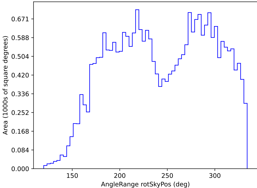
noroll_mjdp270_v3.4_10yrs All sky g band: AngleRange rotSkyPos
