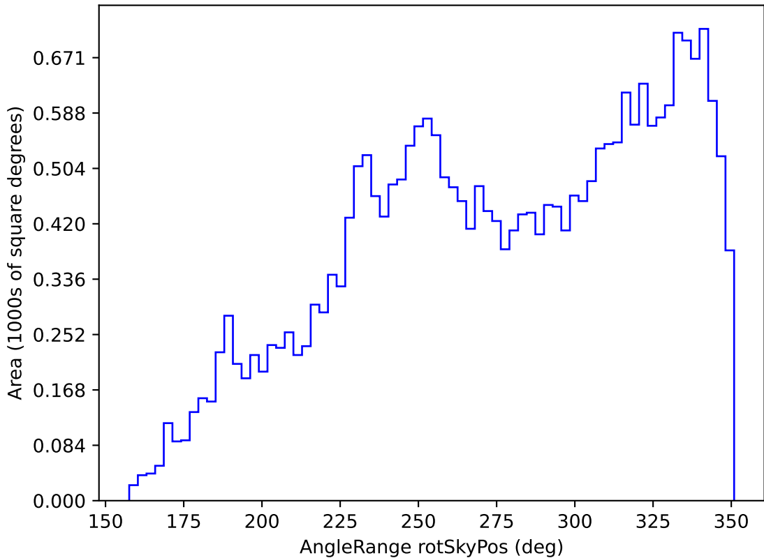
noroll_mjdp270_v3.4_10yrs All sky all bands: AngleRange rotSkyPos
