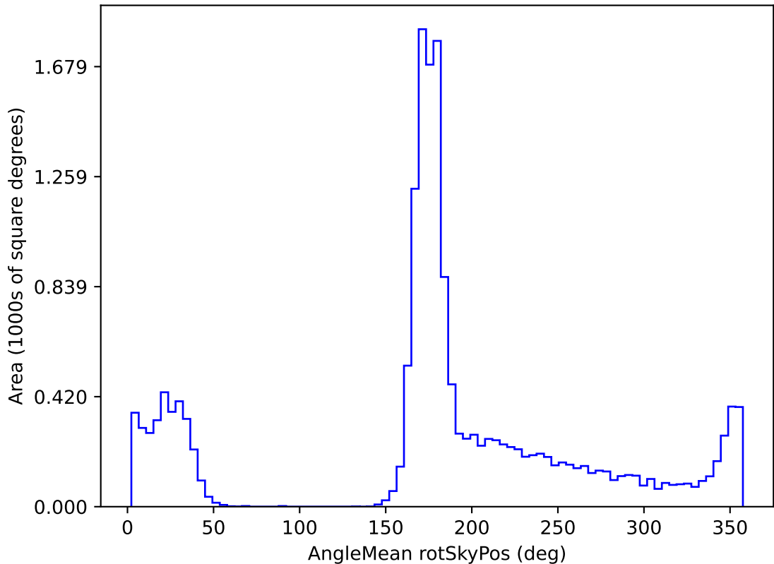
noroll_mjdp270_v3.4_10yrs WFD r band: AngleMean rotSkyPos
