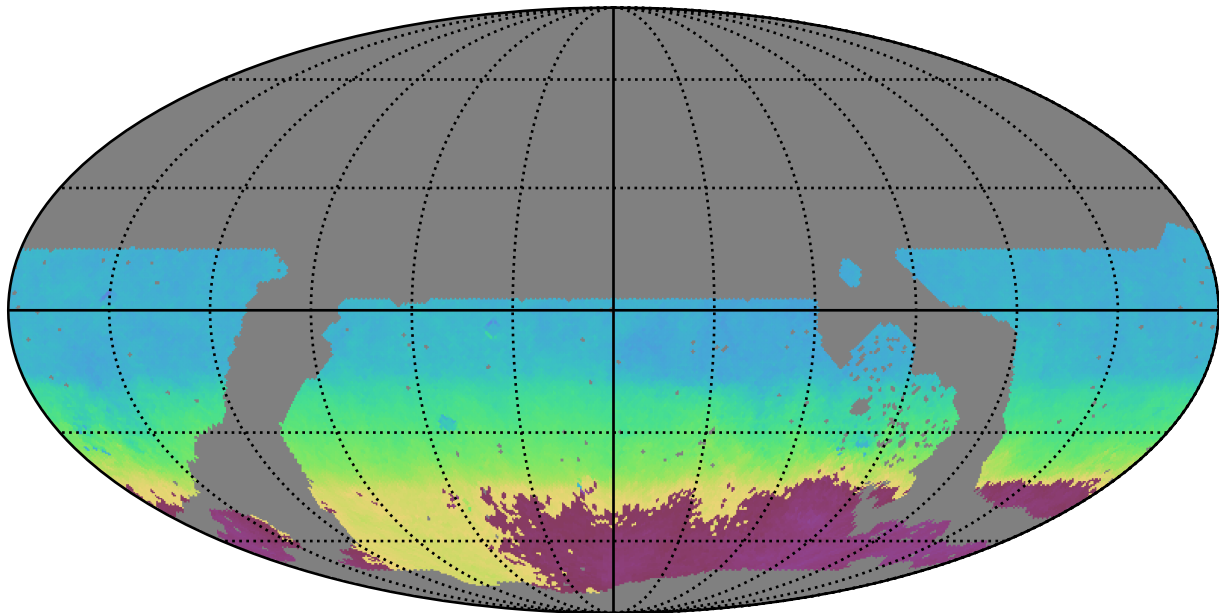
noroll_mjdp270_v3.4_10yrs WFD i band: AngleMean rotSkyPos
