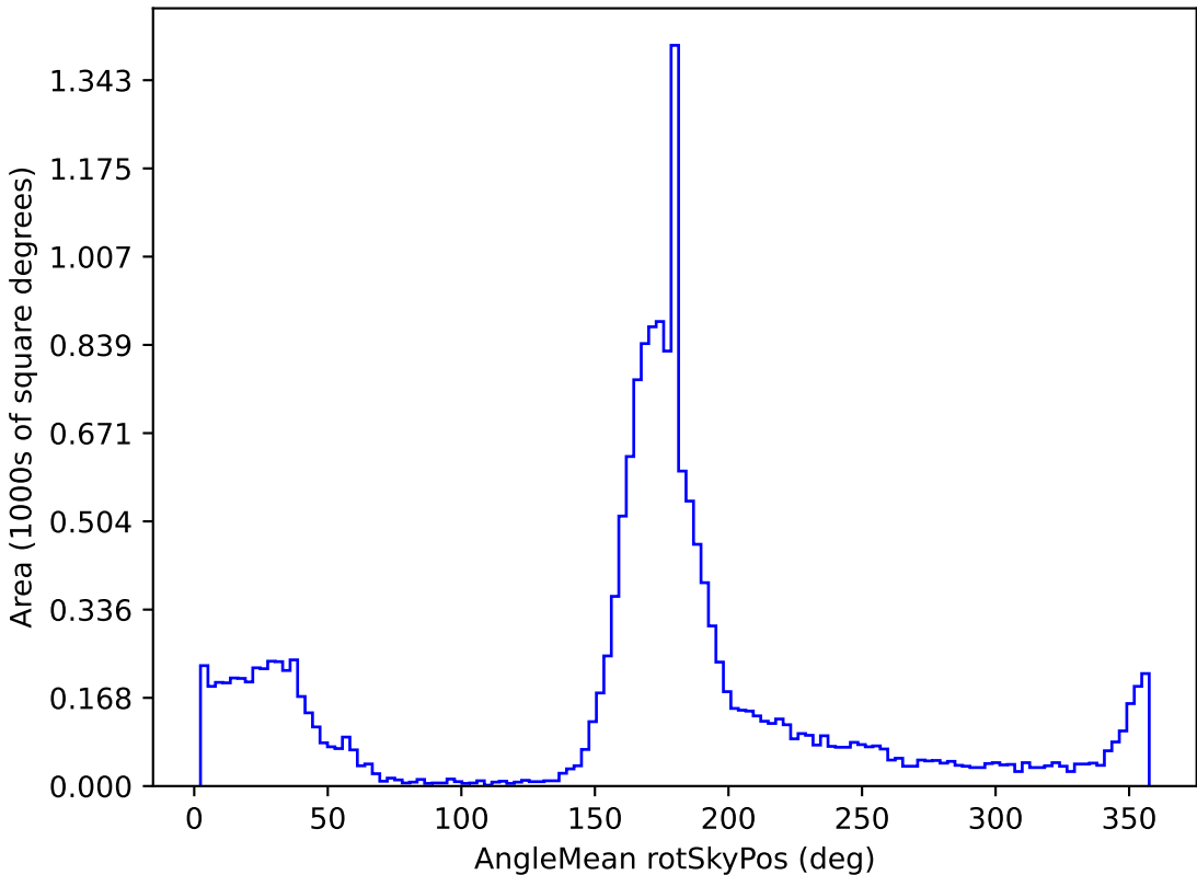
noroll_mjdp270_v3.4_10yrs WFD g band: AngleMean rotSkyPos
