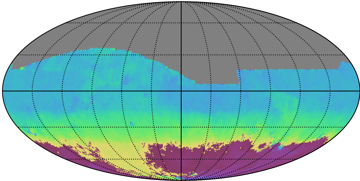
noroll_mjdp270_v3.4_10yrs All sky z band: AngleMean rotSkyPos
