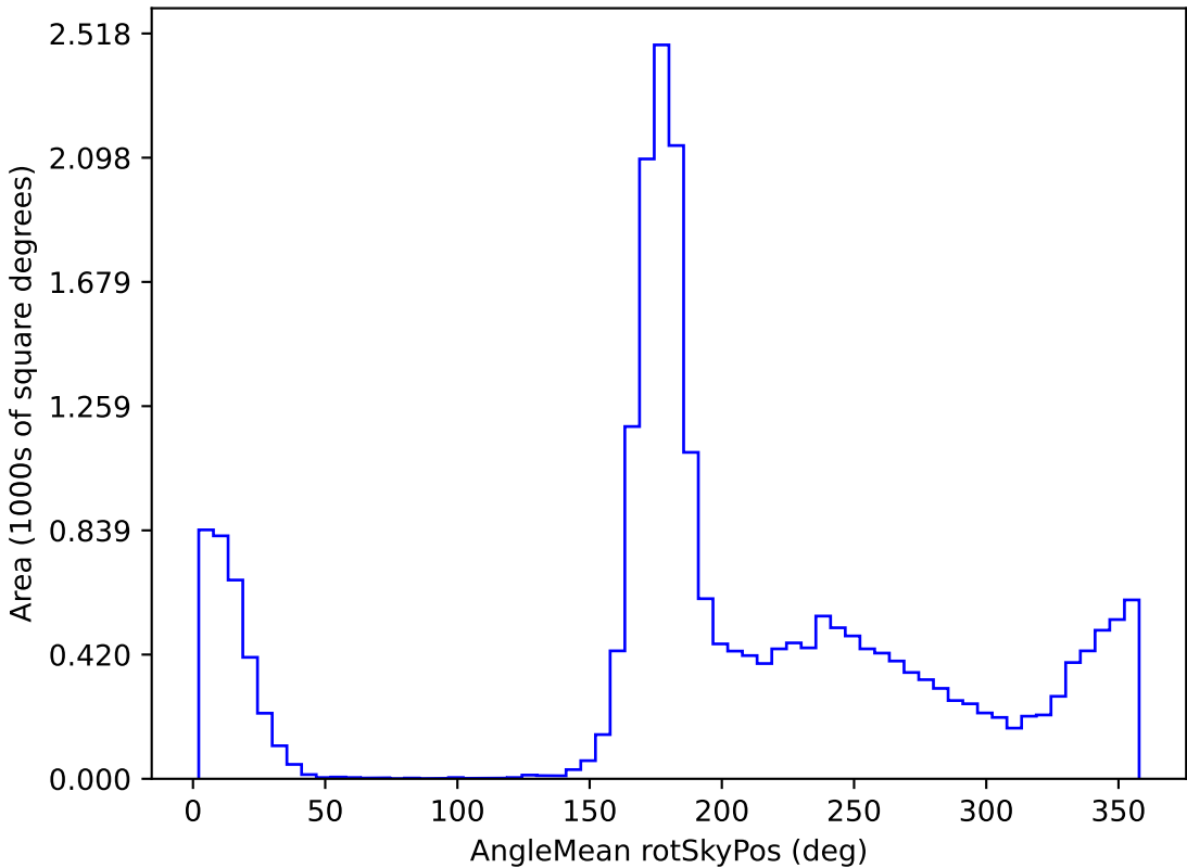
noroll_mjdp270_v3.4_10yrs All sky y band: AngleMean rotSkyPos
