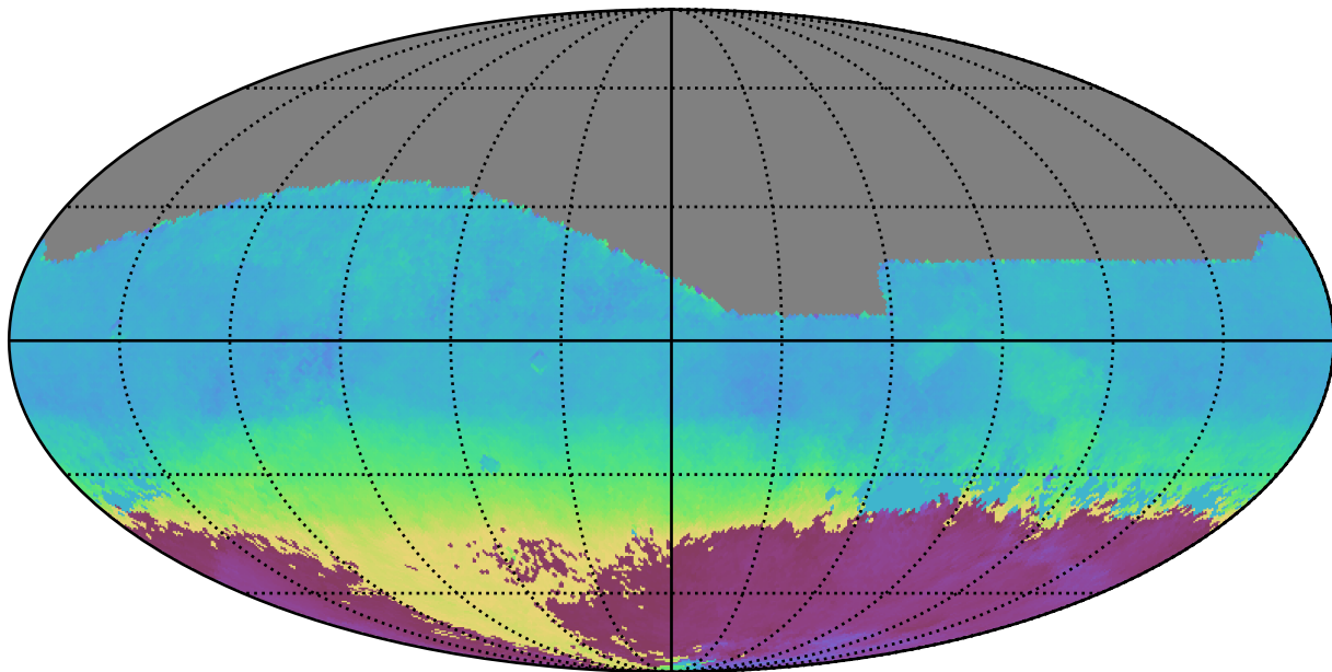
noroll_mjdp270_v3.4_10yrs All sky r band: AngleMean rotSkyPos
