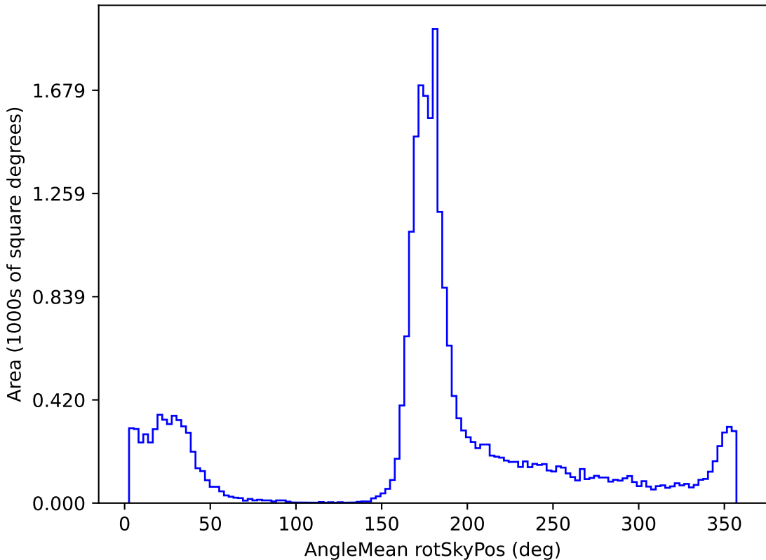
noroll_mjdp270_v3.4_10yrs All sky r band: AngleMean rotSkyPos
