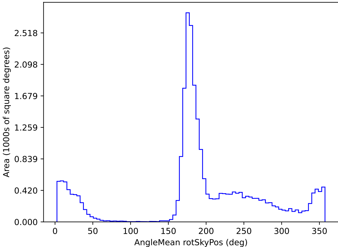
noroll_mjdp270_v3.4_10yrs All sky i band: AngleMean rotSkyPos
