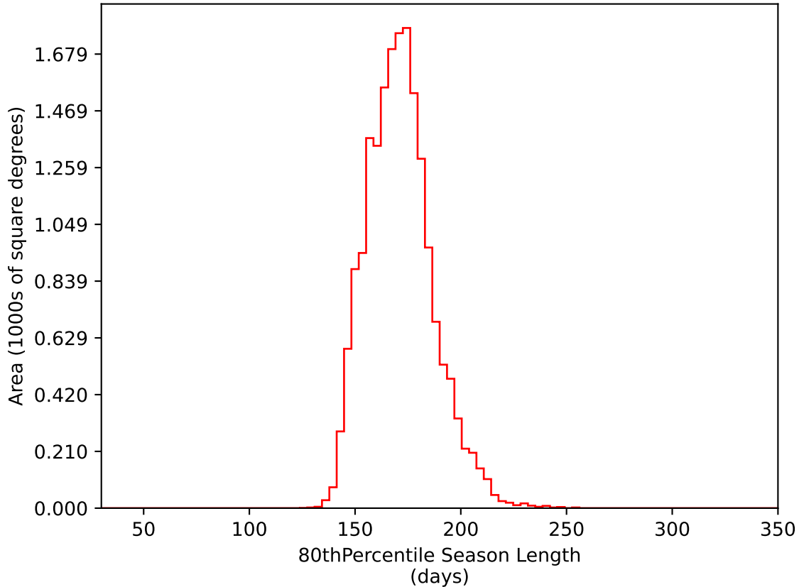
noroll_mjdp270_v3.4_10yrs WFD i band: 80thPercentile Season Length
