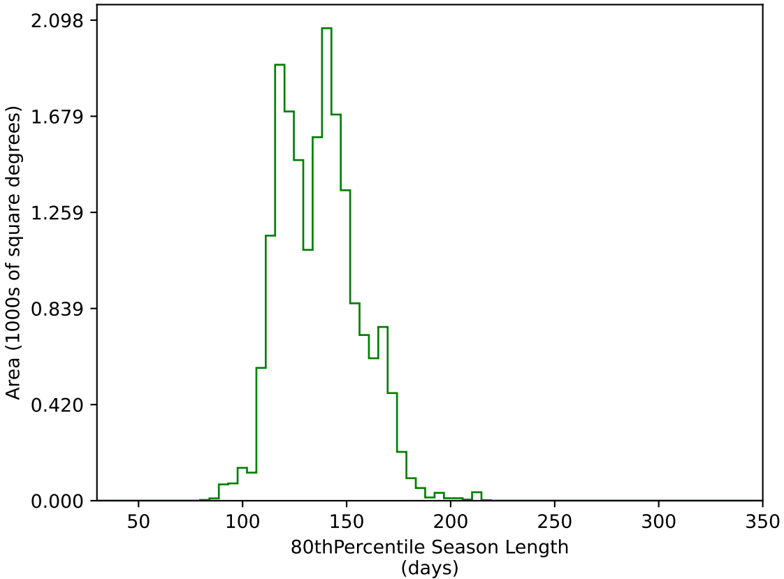
noroll_mjdp270_v3.4_10yrs WFD g band: 80thPercentile Season Length
