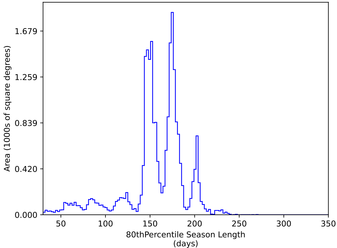
noroll_mjdp270_v3.4_10yrs All sky y band: 80thPercentile Season Length
