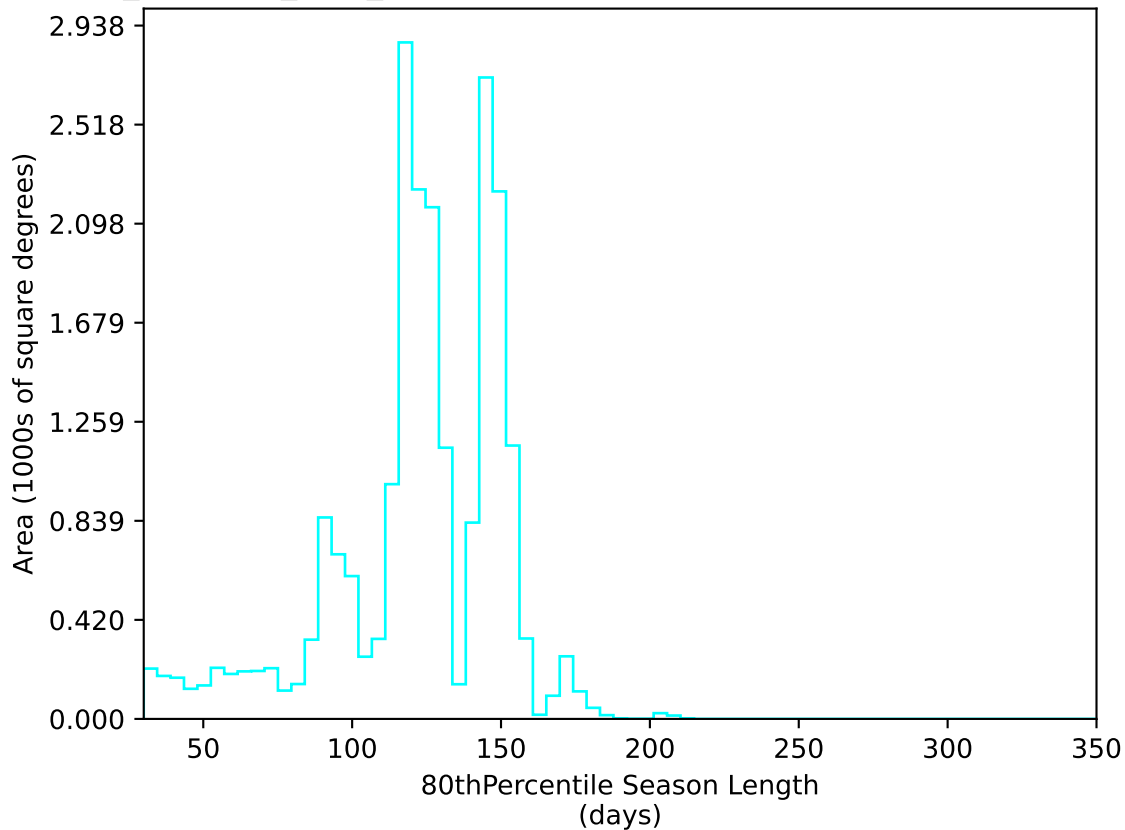
noroll_mjdp270_v3.4_10yrs All sky u band: 80thPercentile Season Length
