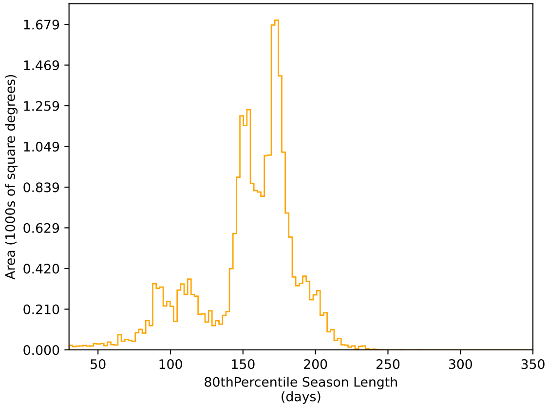
noroll_mjdp270_v3.4_10yrs All sky r band: 80thPercentile Season Length
