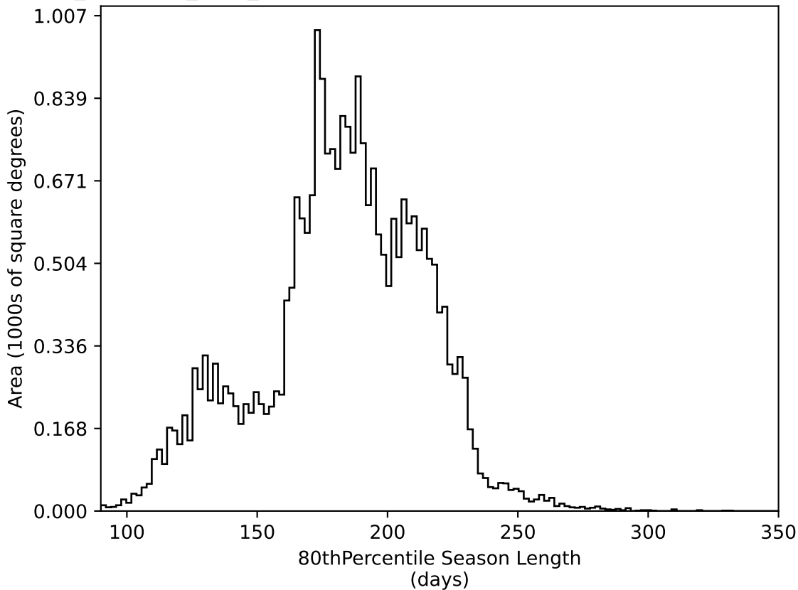
noroll_mjdp270_v3.4_10yrs All sky all bands: 80thPercentile Season Length
