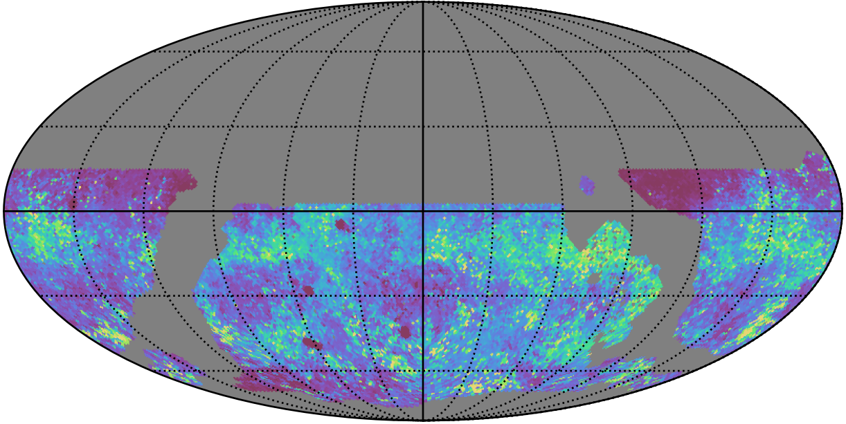
noroll_mjdp270_v3.4_10yrs WFD zy bands: 75th Percentile Intranight Timespan
