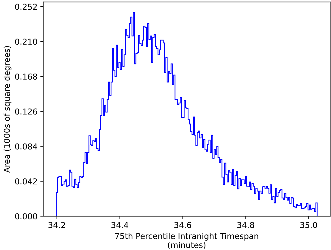
noroll_mjdp270_v3.4_10yrs WFD zy bands: 75th Percentile Intranight Timespan
