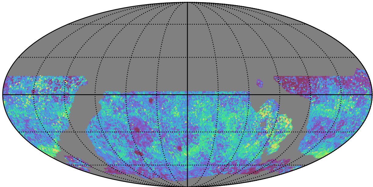
noroll_mjdp270_v3.4_10yrs WFD y band: 75th Percentile Intranight Timespan
