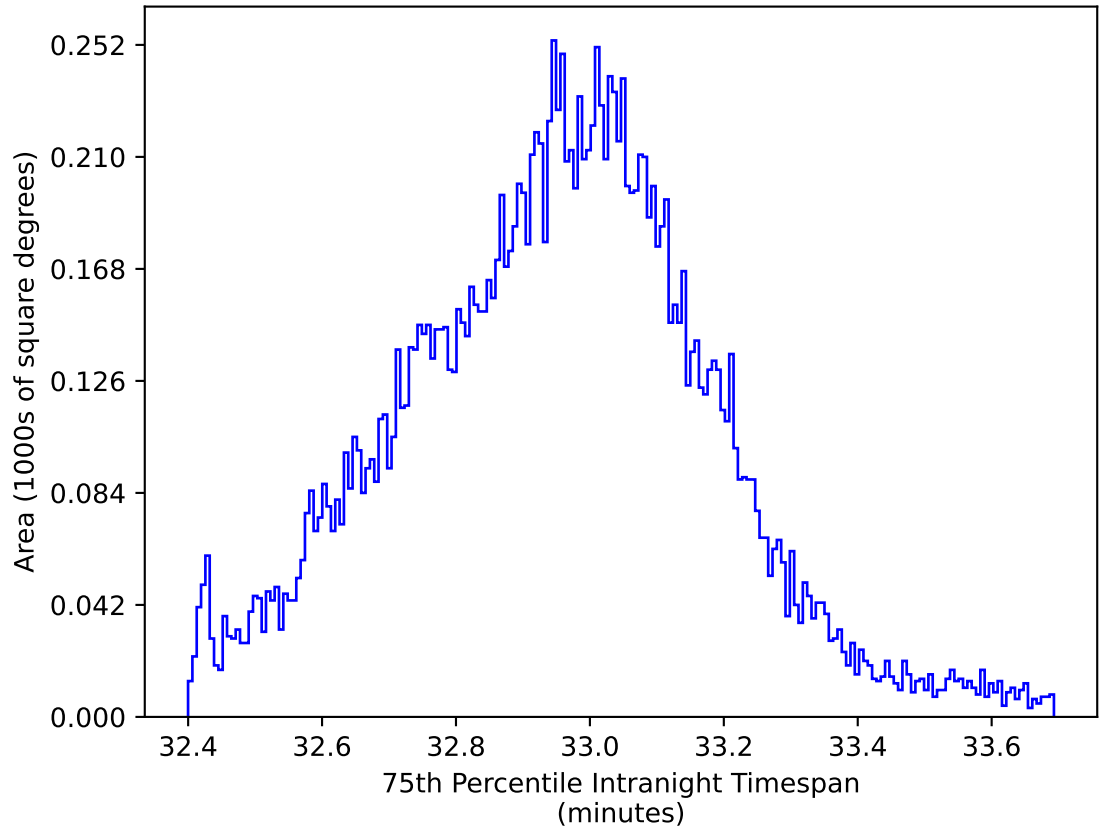
noroll_mjdp270_v3.4_10yrs WFD y band: 75th Percentile Intranight Timespan
