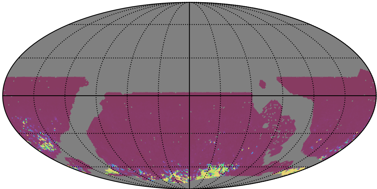
noroll_mjdp270_v3.4_10yrs WFD ri bands: 75th Percentile Intranight Timespan
