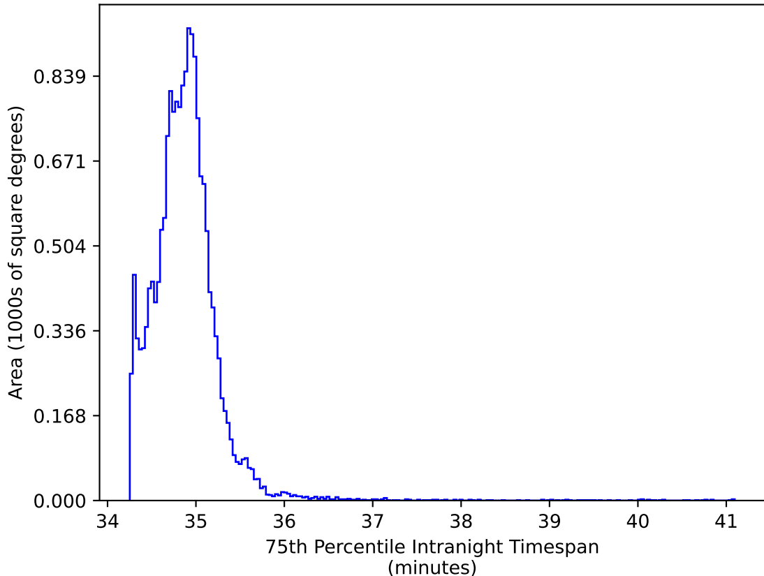
noroll_mjdp270_v3.4_10yrs WFD iz bands: 75th Percentile Intranight Timespan
