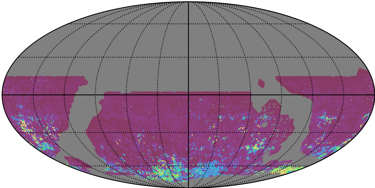
noroll_mjdp270_v3.4_10yrs WFD i band: 75th Percentile Intranight Timespan
