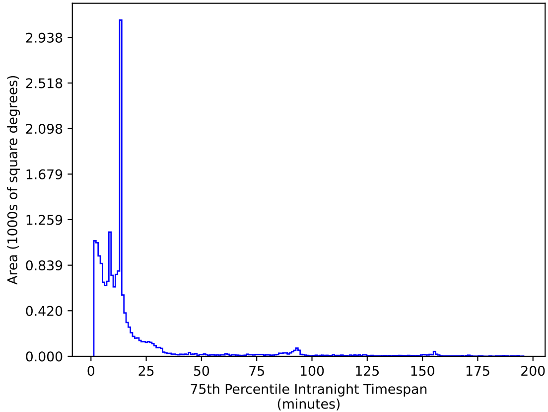
noroll_mjdp270_v3.4_10yrs WFD i band: 75th Percentile Intranight Timespan
