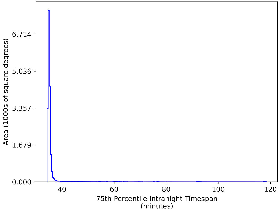
noroll_mjdp270_v3.4_10yrs WFD gr bands: 75th Percentile Intranight Timespan
