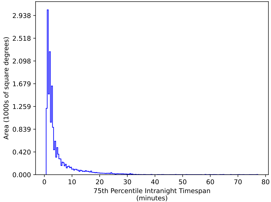
noroll_mjdp270_v3.4_10yrs WFD g band: 75th Percentile Intranight Timespan
