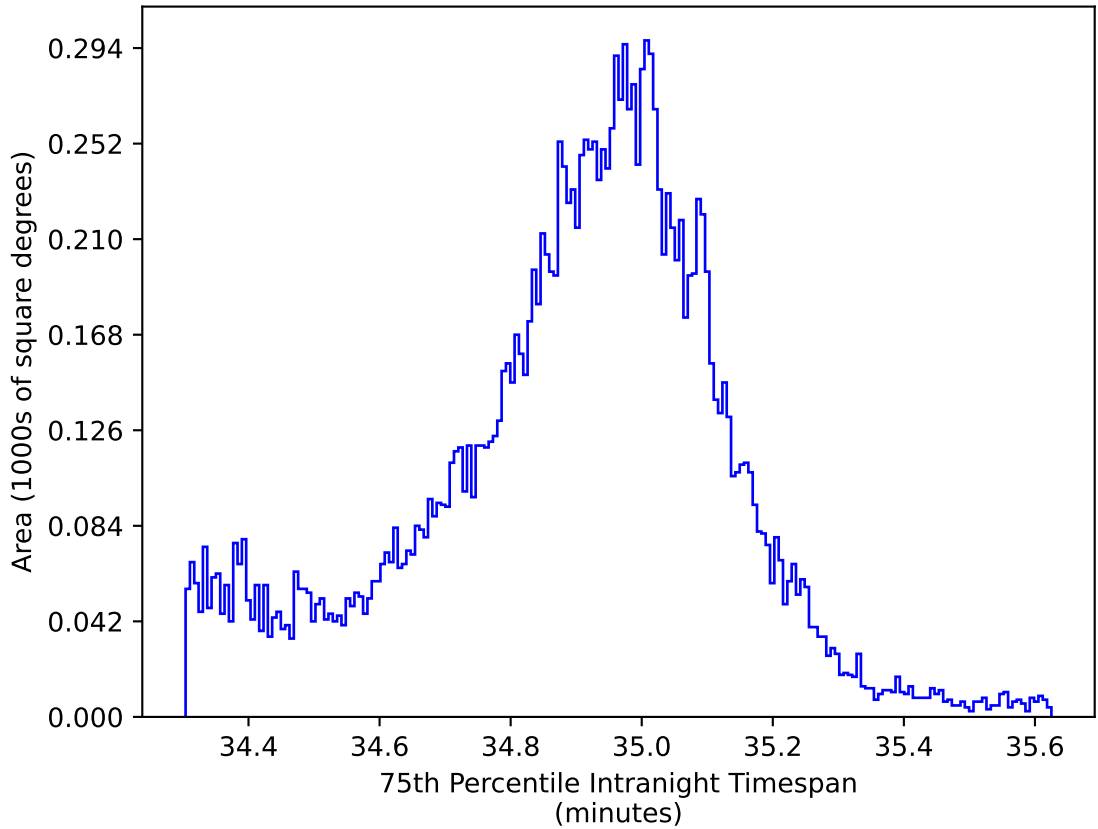
noroll_mjdp270_v3.4_10yrs WFD all bands: 75th Percentile Intranight Timespan
