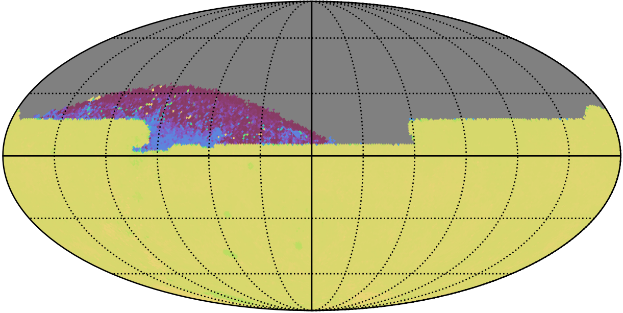
noroll_mjdp270_v3.4_10yrs All sky zy bands: 75th Percentile Intranight Timespan
