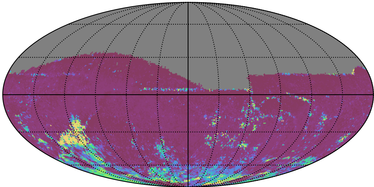
noroll_mjdp270_v3.4_10yrs All sky z band: 75th Percentile Intranight Timespan
