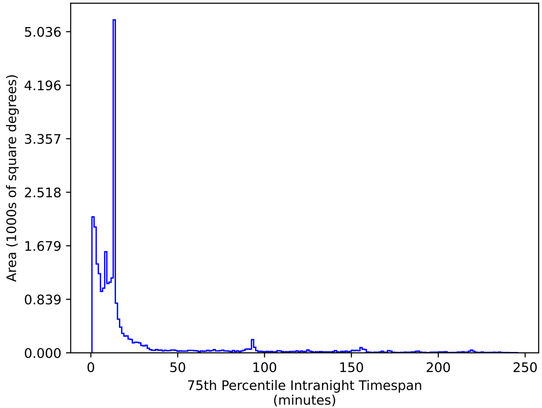
noroll_mjdp270_v3.4_10yrs All sky z band: 75th Percentile Intranight Timespan
