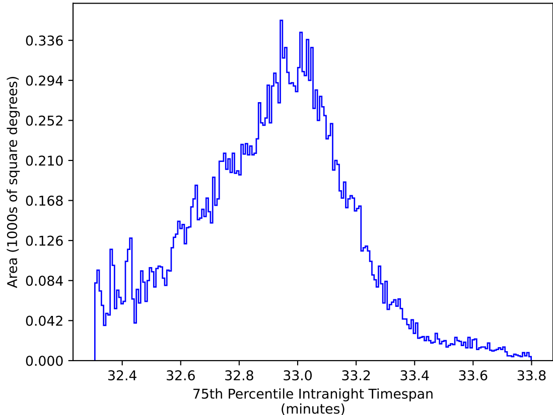
noroll_mjdp270_v3.4_10yrs All sky y band: 75th Percentile Intranight Timespan
