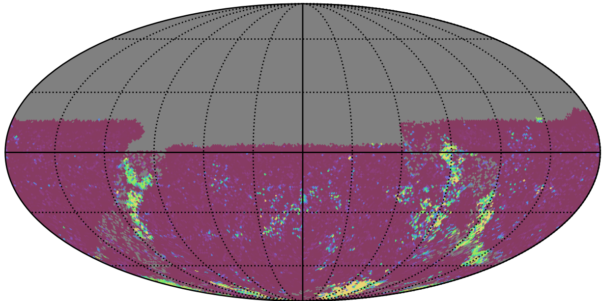
noroll_mjdp270_v3.4_10yrs All sky u band: 75th Percentile Intranight Timespan
